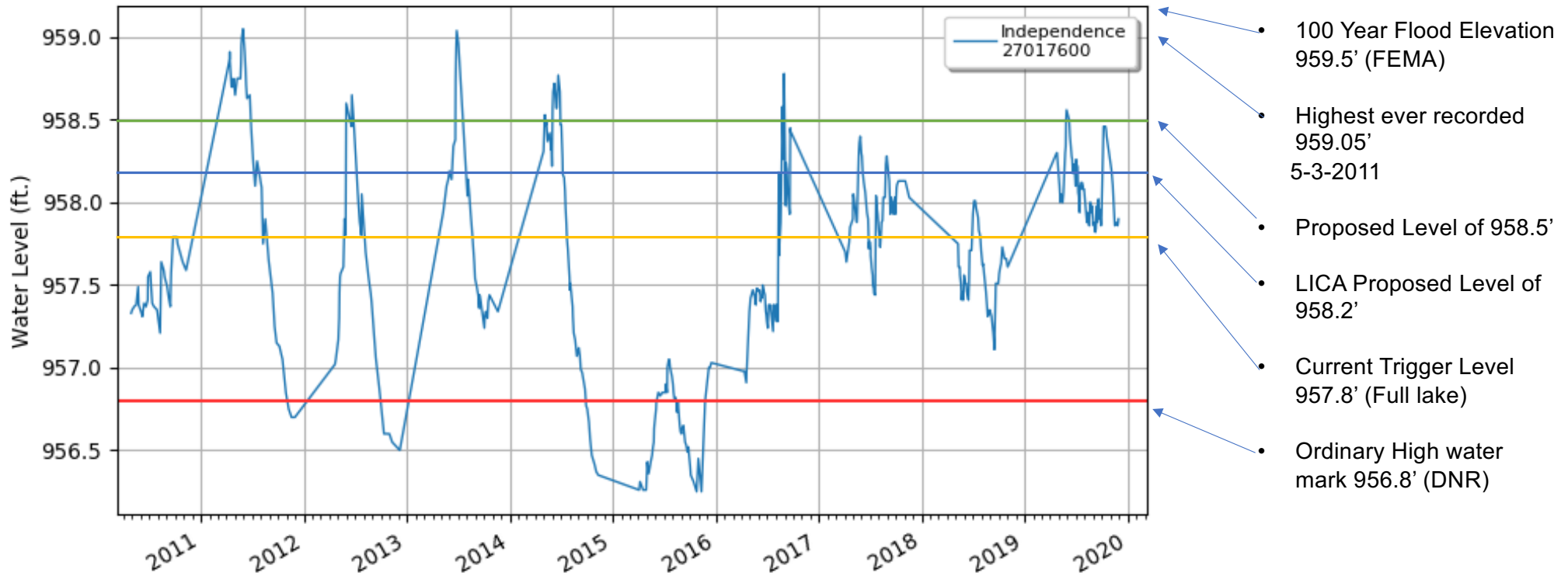
Recorded Water Levels 2010-3-9 to 2020-3-9
